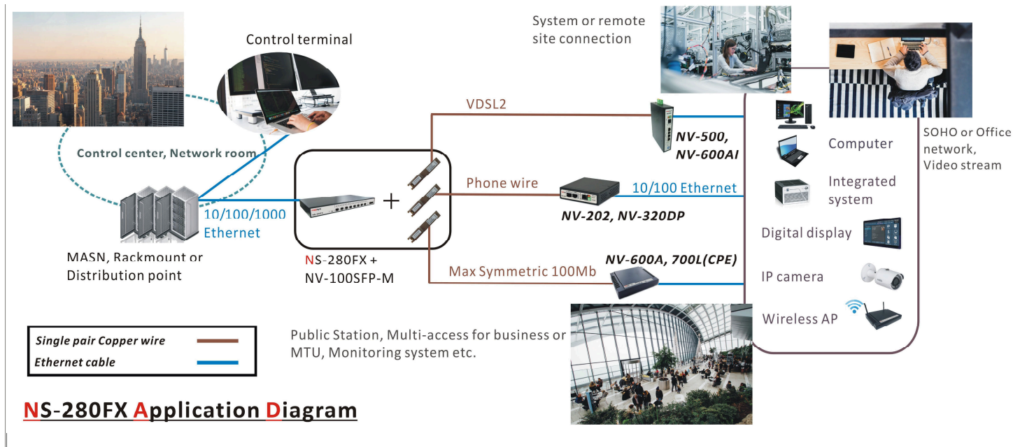
Figure 2.5.1 Application Diagram
